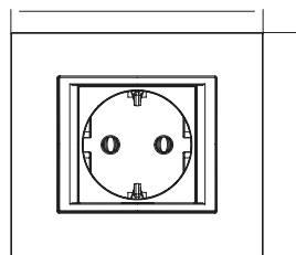
Topraklı Priz Teknik Çizimi Socket Outlet Earthed Technical Drawing
